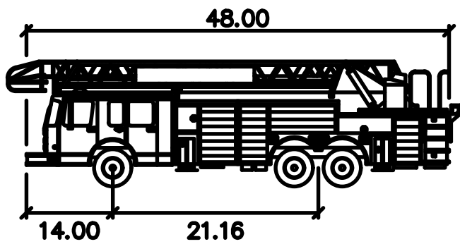
Arlington Heights Fire Truck
