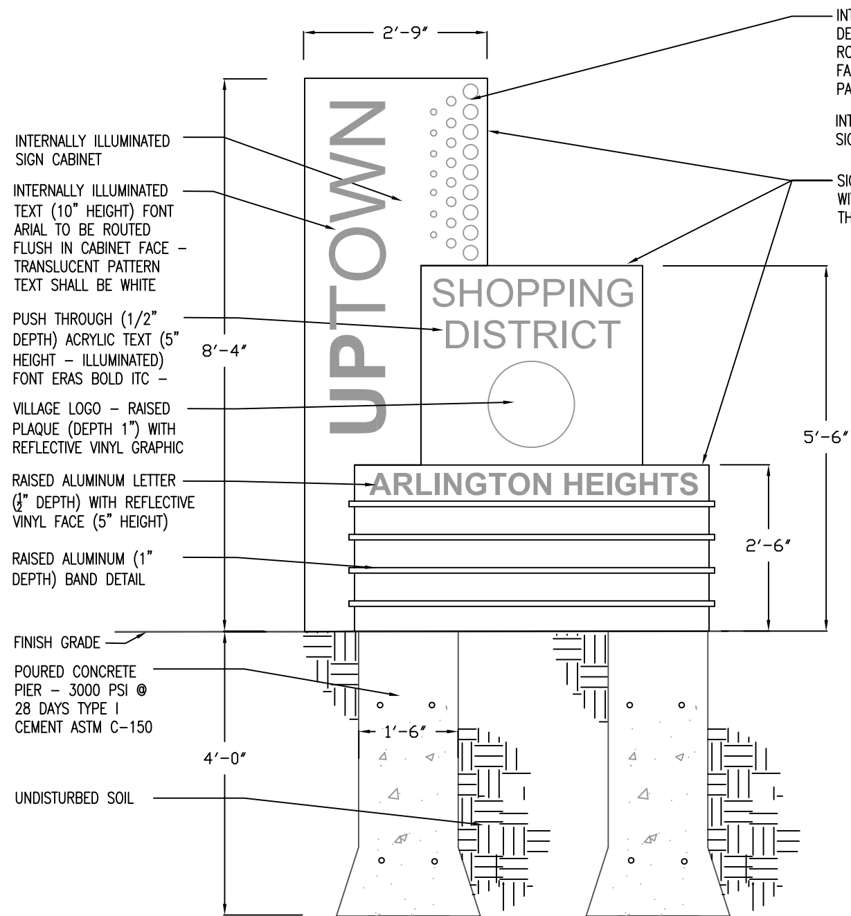
3. FRONT ELEVATION
