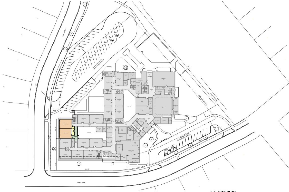
1 SITE PLAN SCALE: 1" = 30'
