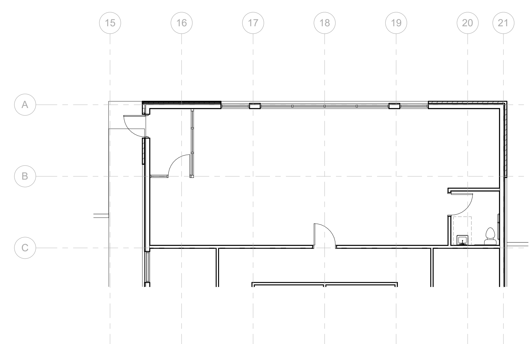
OFFICE PLAN D5 1/8" = 1'-0"
