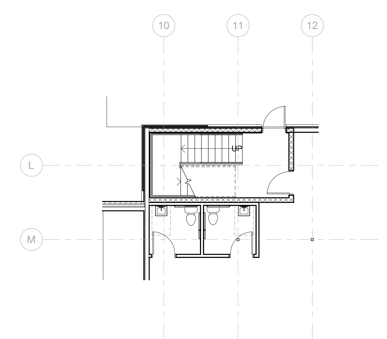
NORTH STAIRS / RESTROOM C5 1/8" = 1'-0"
