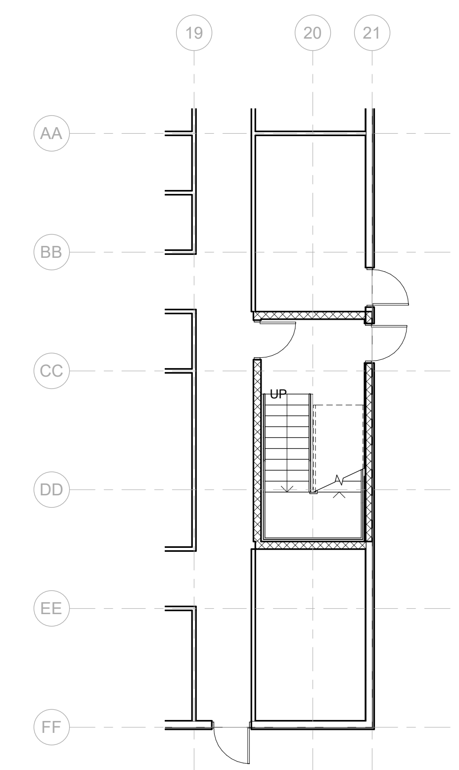
NORTH STAIRS / RESTROOM C5 1/8" = 1'-0"
