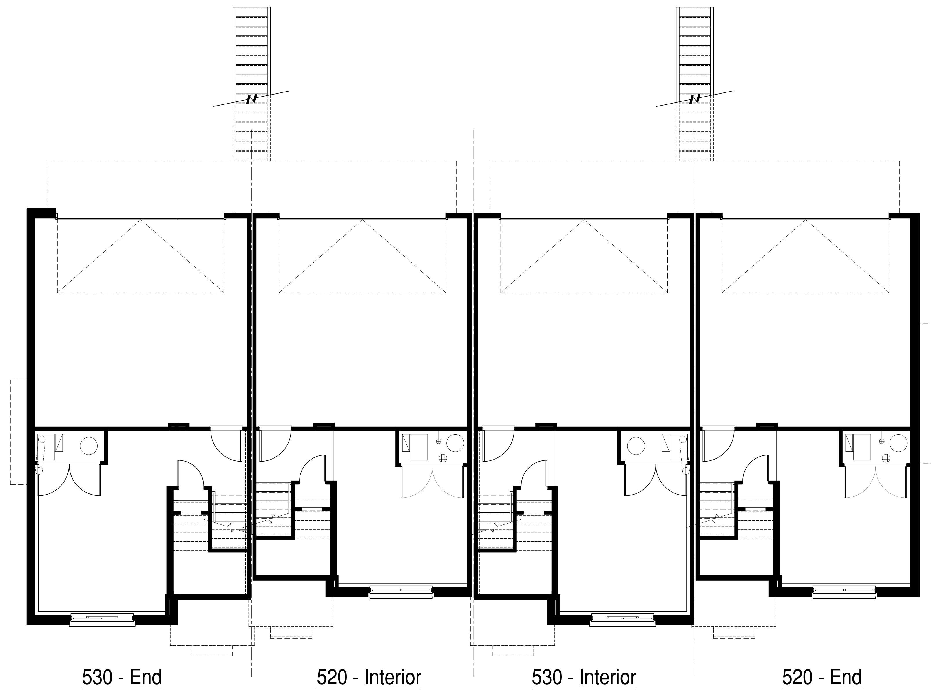
Lower Floor Plan
